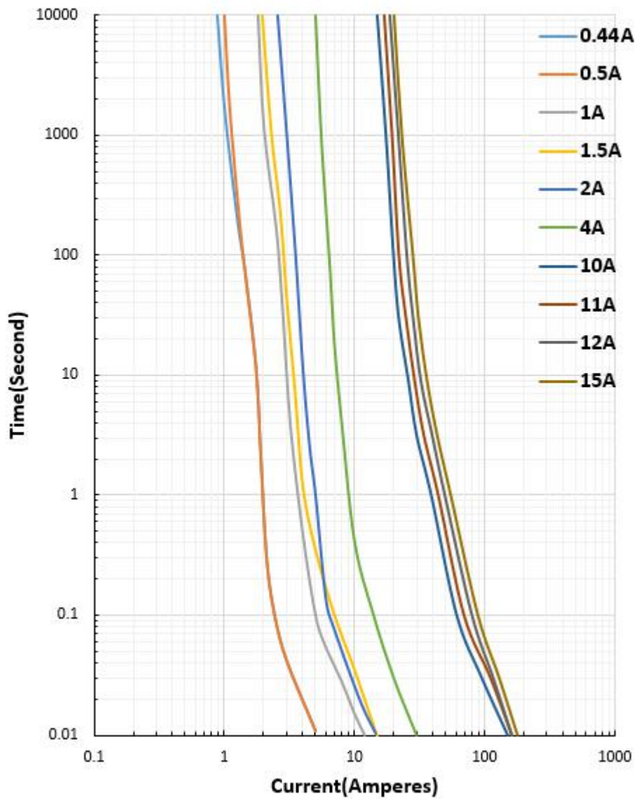
Time Current Curve
